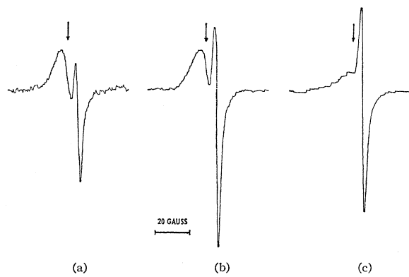
FIG. 6. Electron spin resonance signals of ZnO-B and ZnO-B' obtained from ZnO:10 -2 NaCl at 77°K with three different microwave power levels: (a) 1 mW, (b) 4 mW, and (c) 16 mW. The relative settings of the amplifier gain were 4, 2.6, and 1 for the spectra (a), (b), and (c), respectively. The arrows indicate the points corresponding to g=1.960 , and the field increases from left to right.
