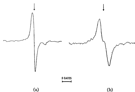
FIG. 8. Electron spin resonance signals of ZnO- B' centers obtained at 180°K from (a) ZnO:10 -2 KCl and (b) ZnO:10 -2 KF. The arrows indicate the points corresponding to g=1.960 , and the field increases from left to right.
