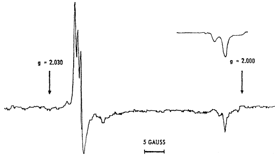
FIG. 3. Electron spin resonance signal obtained from ZnO:10 -3 Li 6 Cl (90% enriched) at 77°K under uv excitation. The figure at the upper right corner shows the high-field signal ( \theta=0 ) of the same spectrum obtained at slower sweep rate. Note a doublet pattern of the signal.
