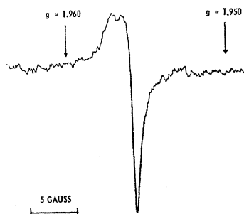
FIG. 4. Electron spin resonance spectra of the g \cong 1.96 region obtained at 77°K without uv illumination from pure ZnO powder that had been fired in air at 900°C.
