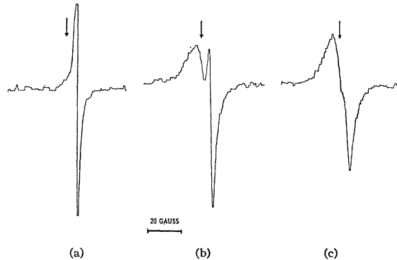
FIG. 5. Electron spin resonance spectra of the g \cong 1.96 region obtained from (a) ZnO, (b) ZnO: 10^{-2} NaCl, and (c) ZnO: 10^{-1} NaCl at 77^\circ K without uv illumination. The arrows indicate the points corresponding to g = 1.960 , and the field increases from left to right.
