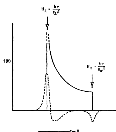
FIG. 1. The shape function S(H) and the derivative curve of the spin resonance absorption expected from polycrystalline sample with g_1 > g_{11} .
