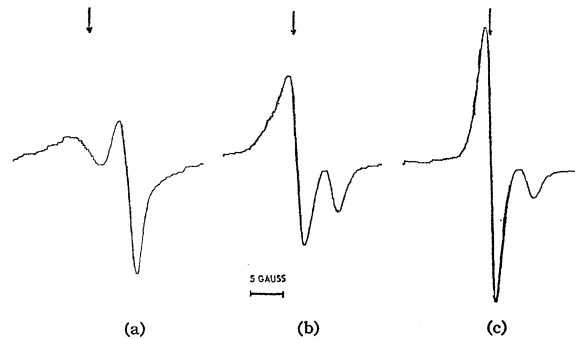
FIG. 7. Electron spin resonance signals of ZnO-B and ZnO-B' obtained from ZnO:10 -2 NaCl at three different temperatures: (a) 77°K, (b) 110°K, and (c) 140°K. The power level was kept at 4 mW. The arrows indicate the points corresponding to g=1.960 , and the field increases from left to right.
