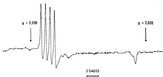
FIG. 2. Electron spin resonance signal obtained from \text{ZnO}:10^{-3} \text{LiCl} at 77^\circ\text{K} under uv excitation.
